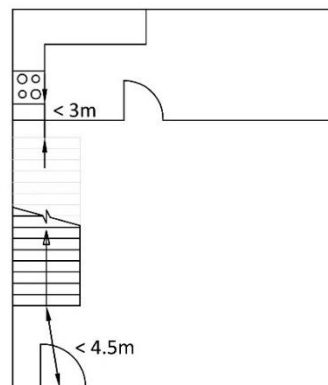
(c) Open plan arrangement for escape - kitchen is enclosed
