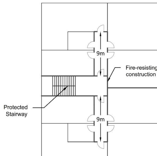
(b) Single stair building containing flats (1 - 2 flats per floor)
