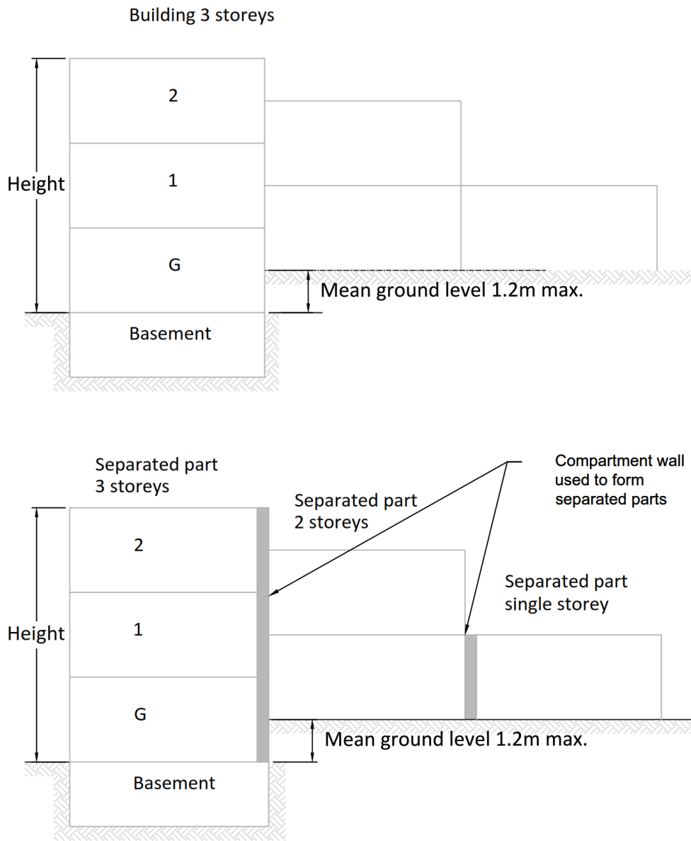
Diagram 89 Number of Storeys
