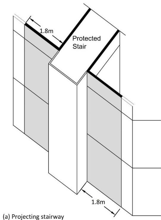
Diagram 15 External Protection to Protected Stairway
