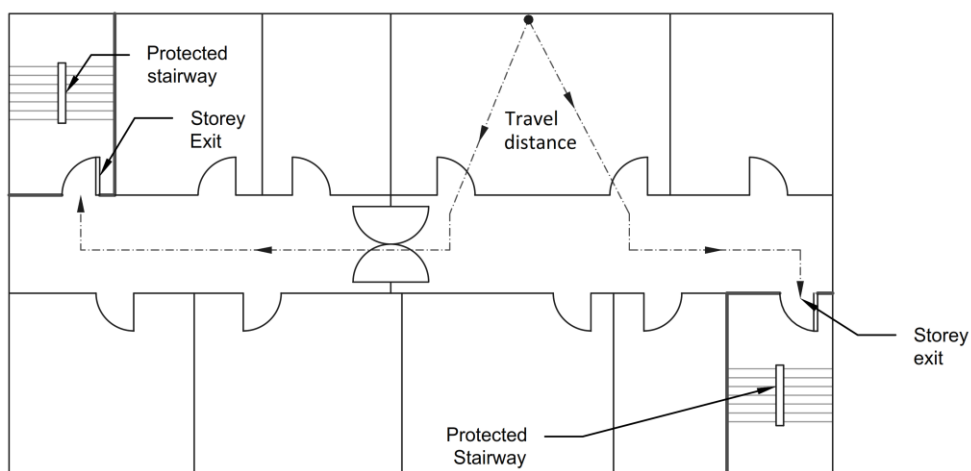
(c) Escape in more than one direction
