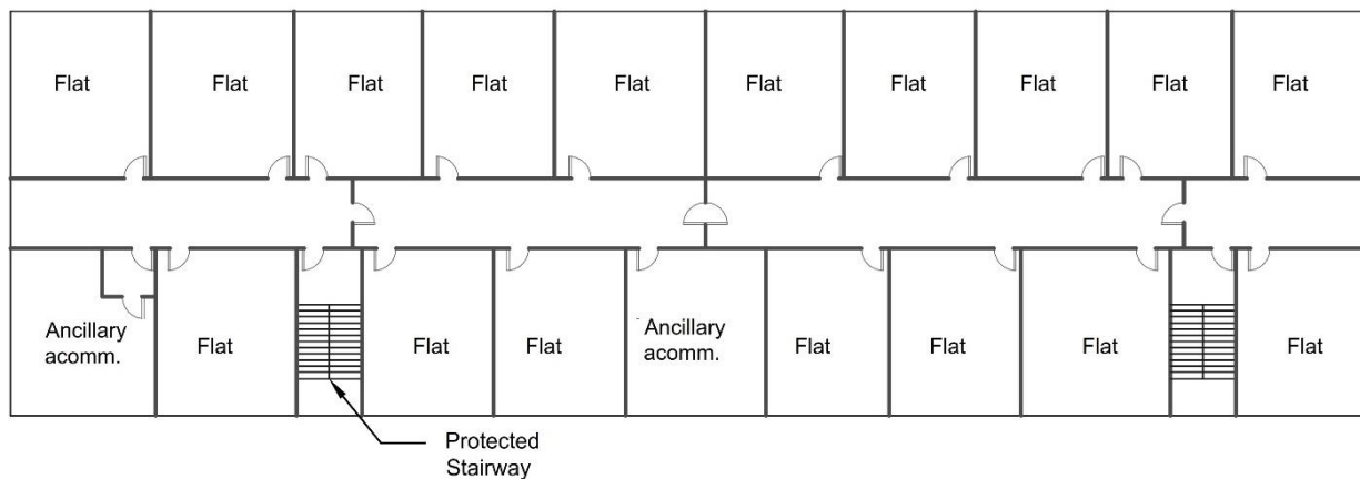
Diagram 32 Ancillary Accommodation in Buildings Containing Flats Para 1.6.8
