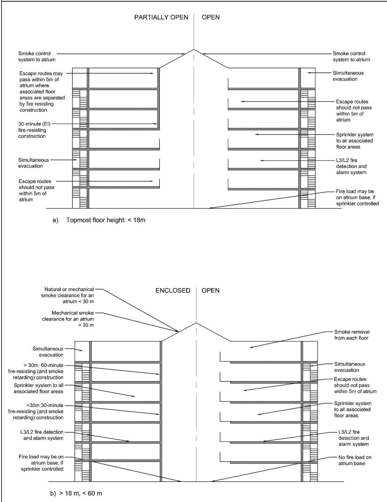
Diagram 61 Atrium in a Shop, Assembly and Recreation or Other Non-residential Building
