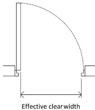
Diagram 80 Measurement of Door Width in Existing Buildings
