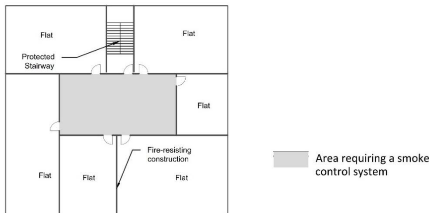
(c) Single stair building containing flats with protected lobby approach
