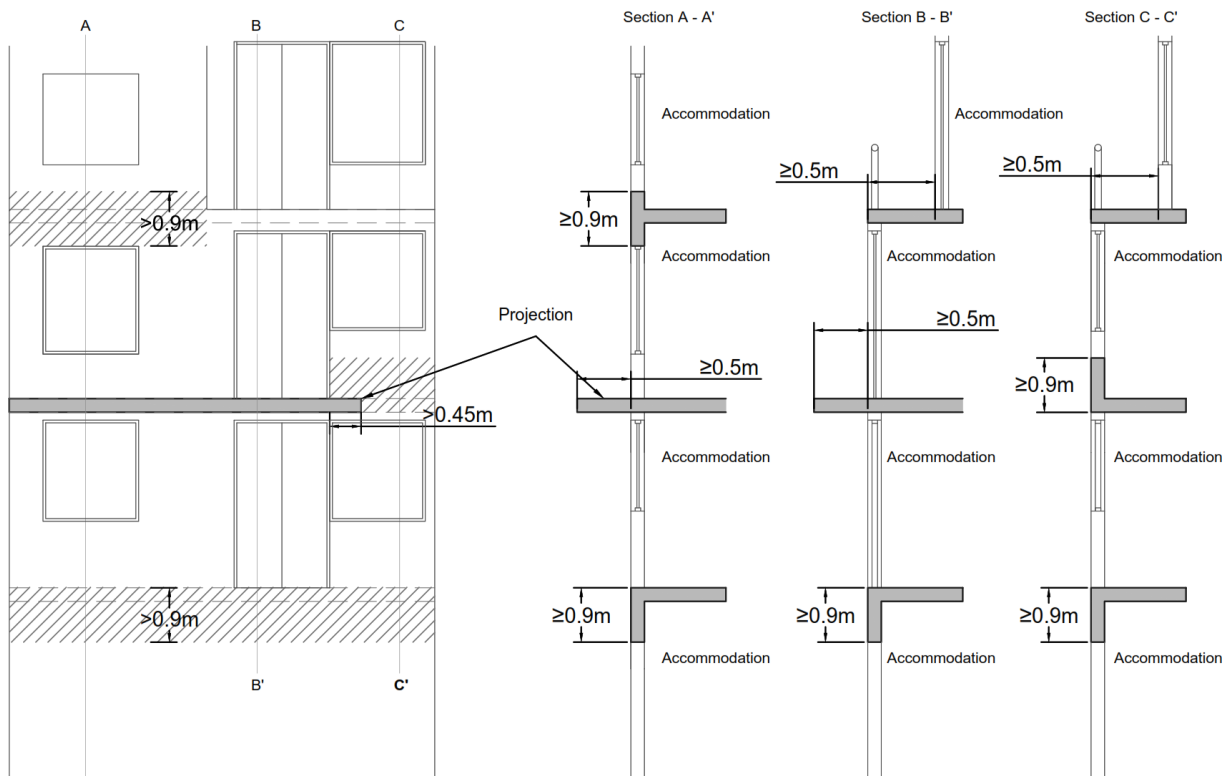
Diagram 48 Junction of a Compartment Floor With an External Wall Para 3.5.10
