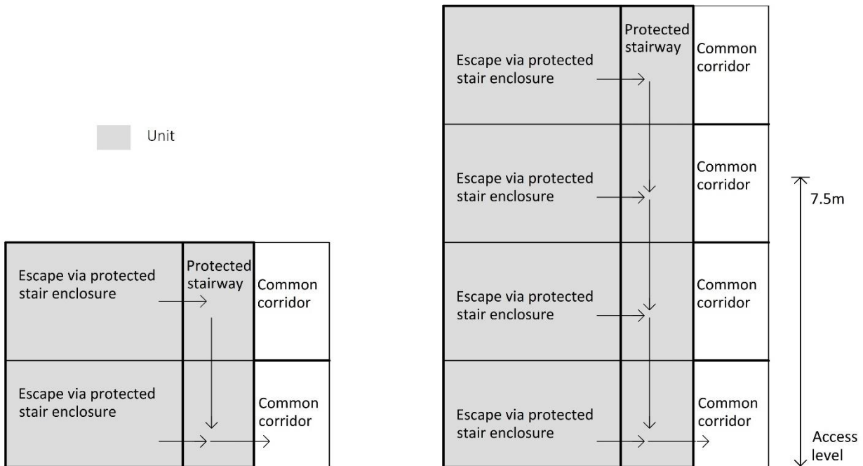
(b) Maisonette with any floor > 4.5 m above ground level
