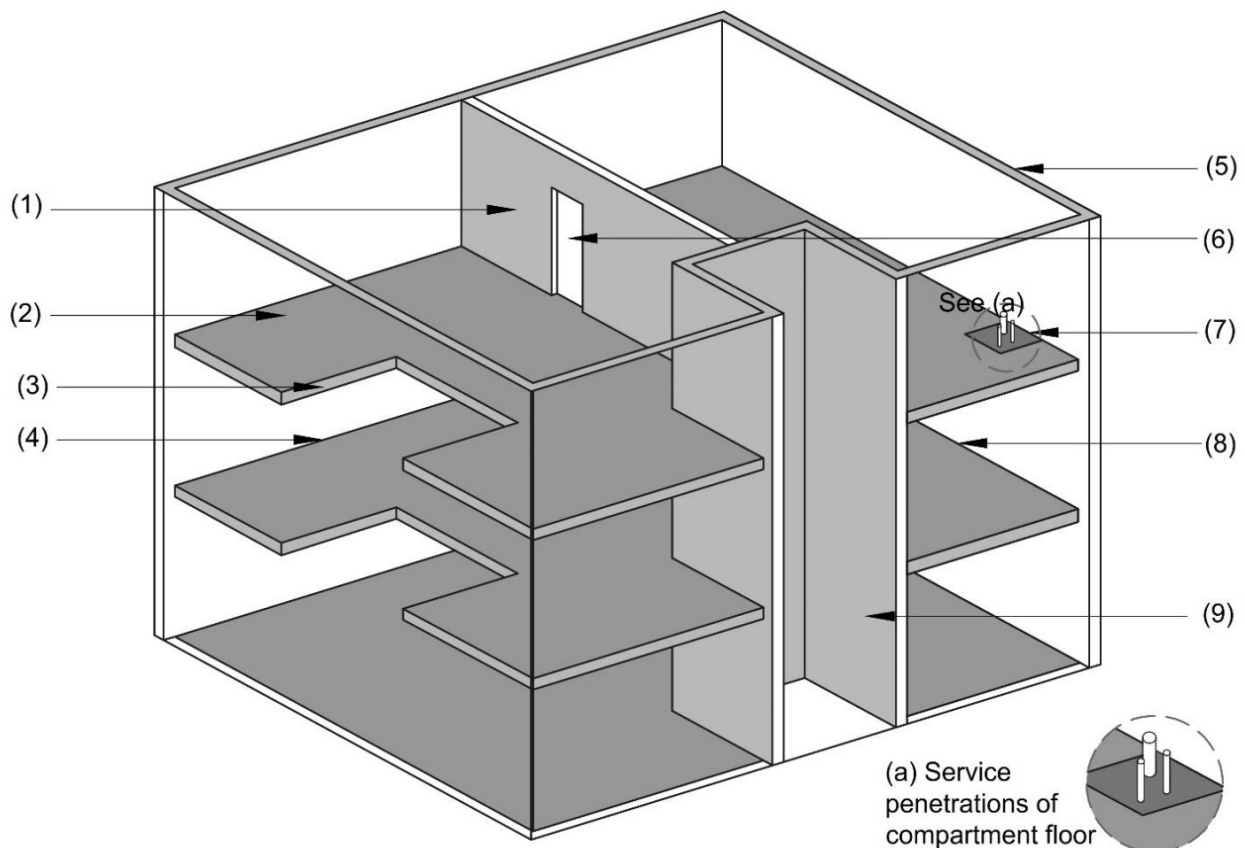
Diagram 46 Compartment Walls and Compartment Floors
