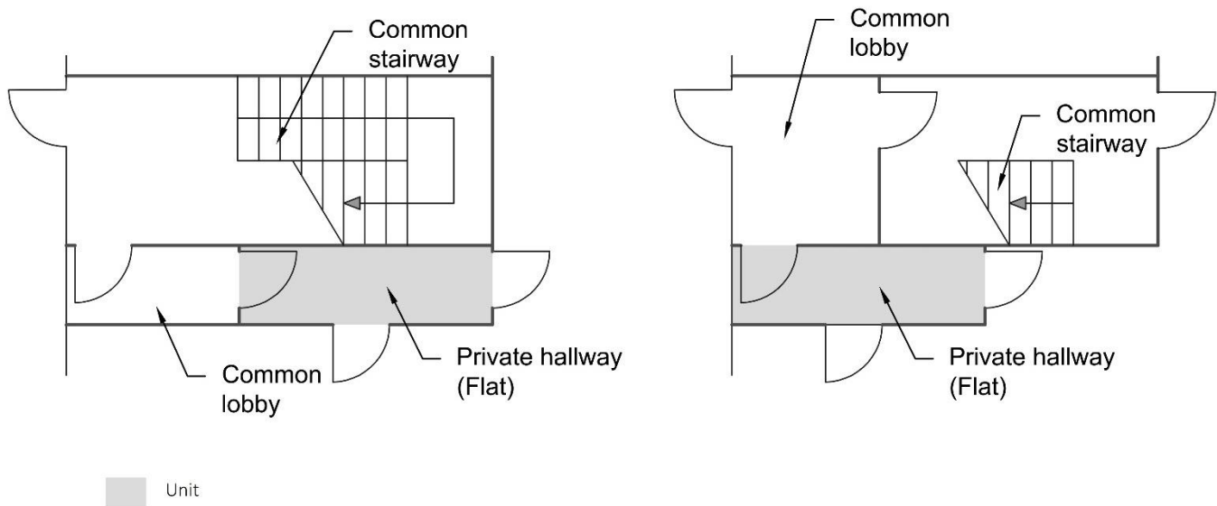
Diagram 31 Final exit from a stairway
