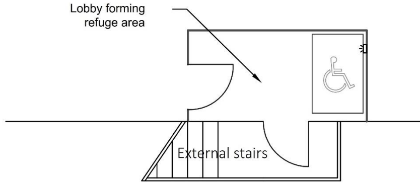
(a) Refuge area provided in a lobby that has direct access to an external escape stair
