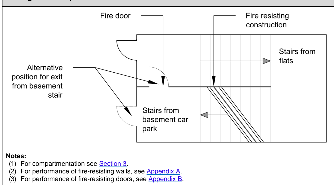
Diagram 26 Separation of Basement Stairs
