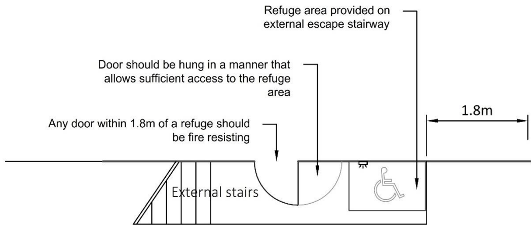
(b) Refuge area provided on an external escape stair
