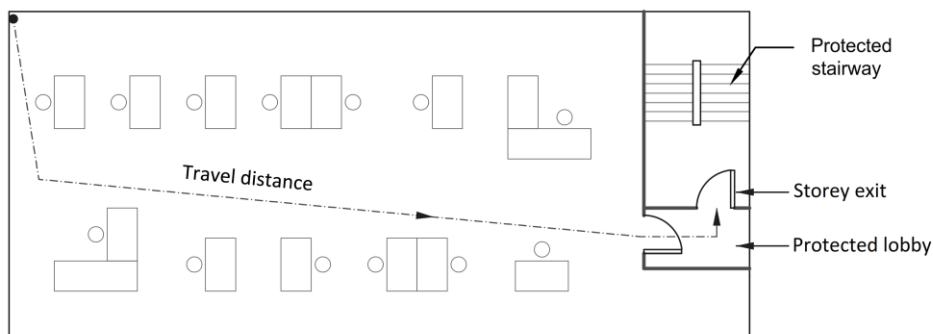
(b) Escape in one direction only (open plan)
