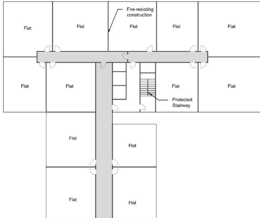
(b) Single stair building containing flats with protected corridor approach
