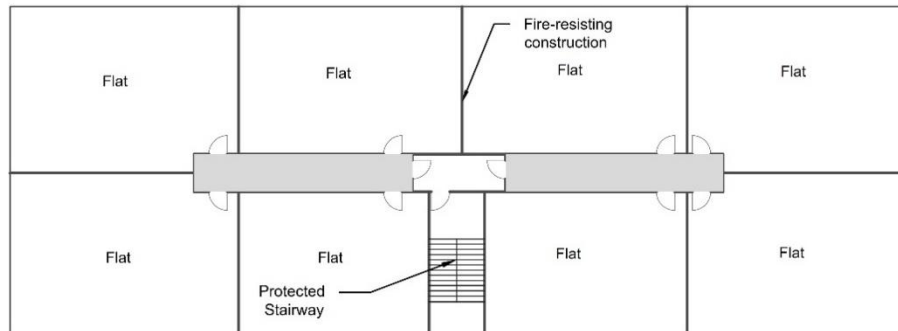
(a) Single stair building containing flats with protected corridor approach
