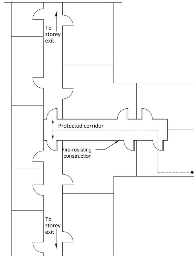
(b) T - Junction with main corridor
