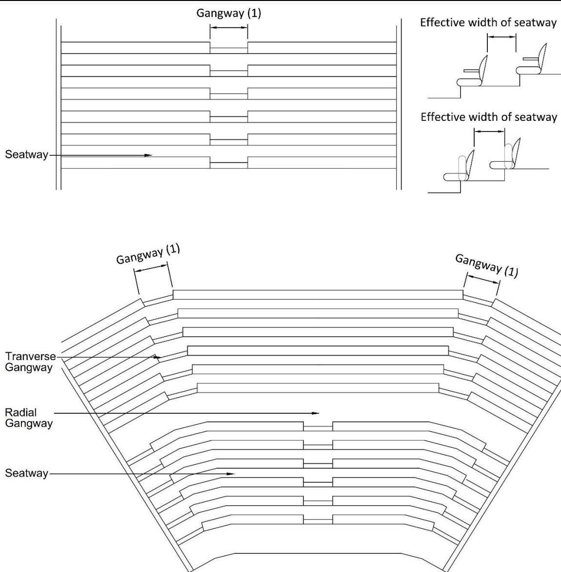
Diagram 12 Seatways and Gangways in Audience and Spectator Facilities Para 1.4.7
