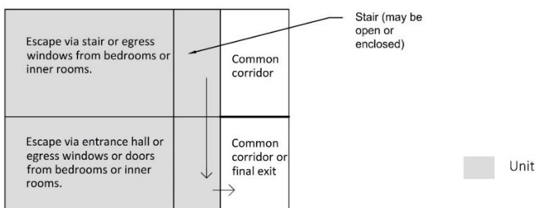
(e) Maisonette with each floor < 4.5 m above ground level
