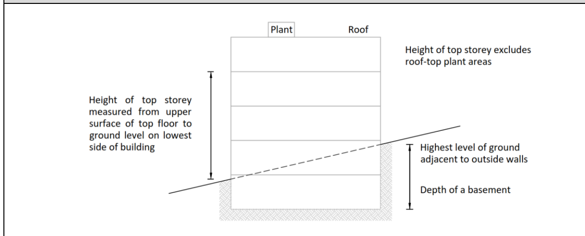
Diagram 91 Height of Top Storey and Depth of a Basement
