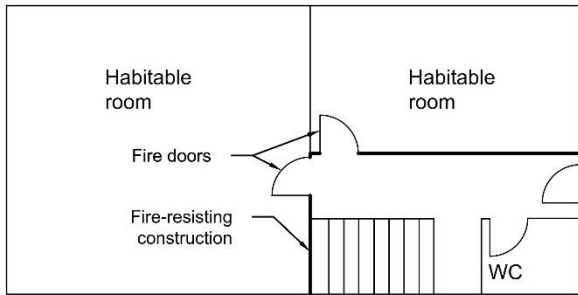
(a) > 4.5m above ground level
