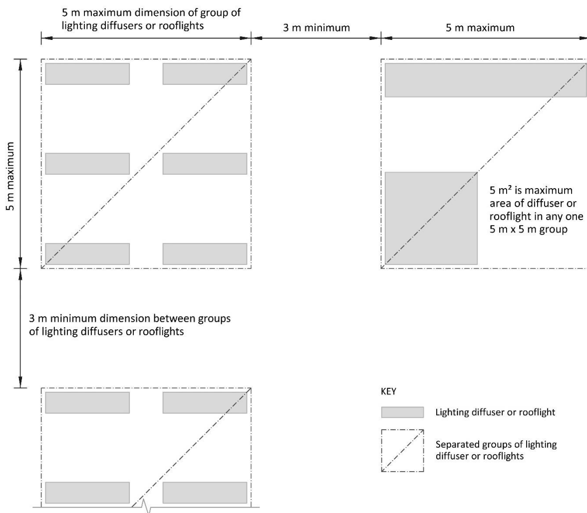
Diagram 44 Layout Restrictions on TP (b) Thermoplastic Lighting Diffusers and Rooflights
