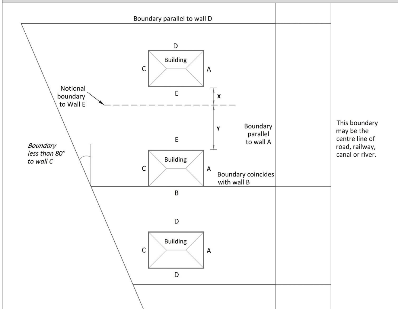
Diagram 65 Relevant & Notional Boundary
