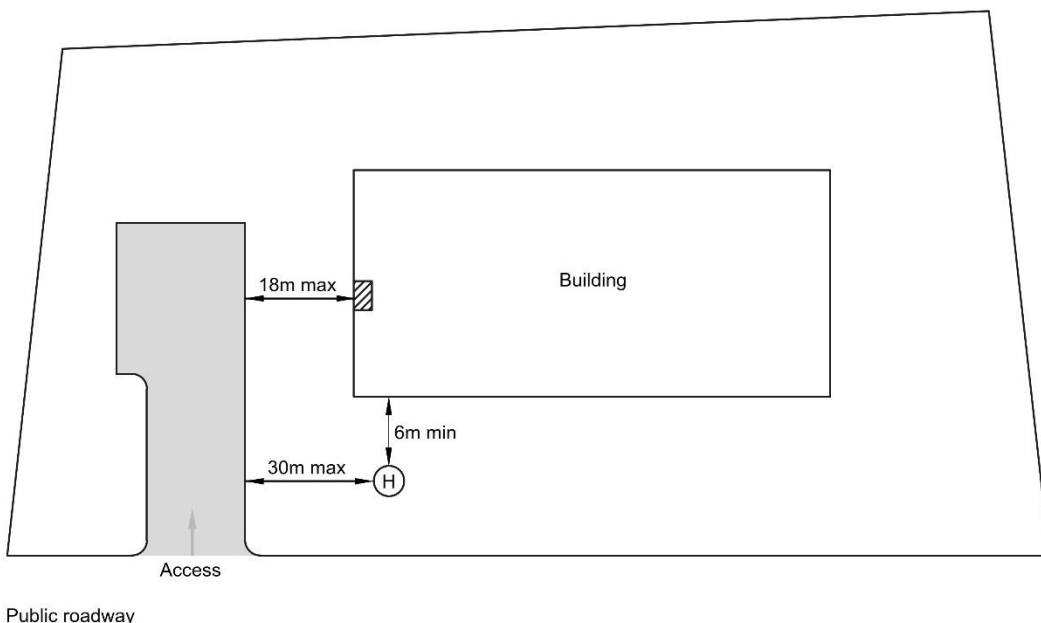
(a) Building with no internal fire main
