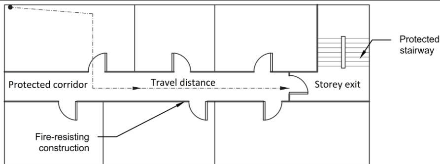
(a) Escape in one direction only (corridor)
