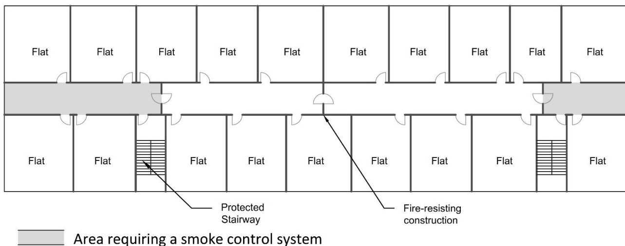
Diagram 29 Flats with a Corridor / Lobby Approach - Multiple Stairs
