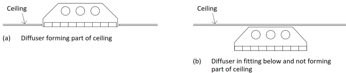
Diagram 44 Layout Restrictions on TP (b) Thermoplastic Lighting Diffusers and Rooflights
