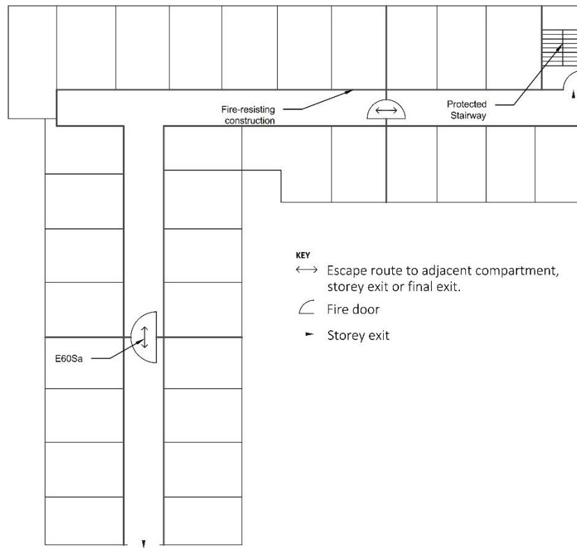
Diagram 11 Progressive Horizontal Evacuation in Residential (Care Facility) Buildings
