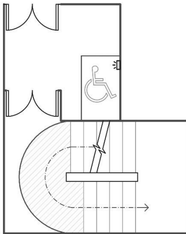
(c) Refuge in protected lobby adjacent to stair
