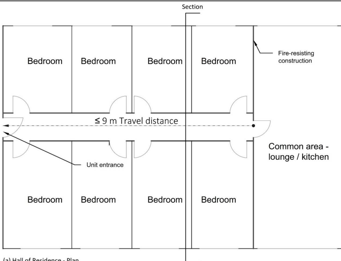
Diagram 13 Student accommodation unit
