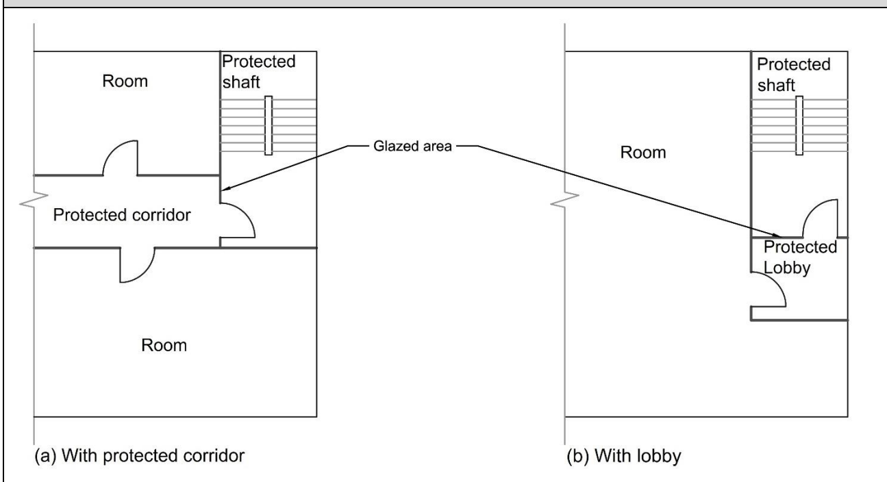
Diagram 52 Glazed Screen Separating Protected Shaft From Lobby Para 3.5.16.3.1 or Corridor
