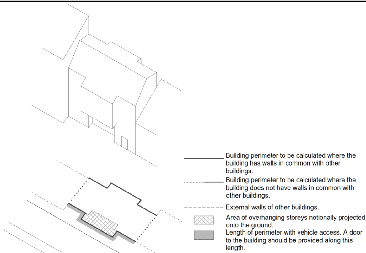
Diagram 72 Building Perimeter
