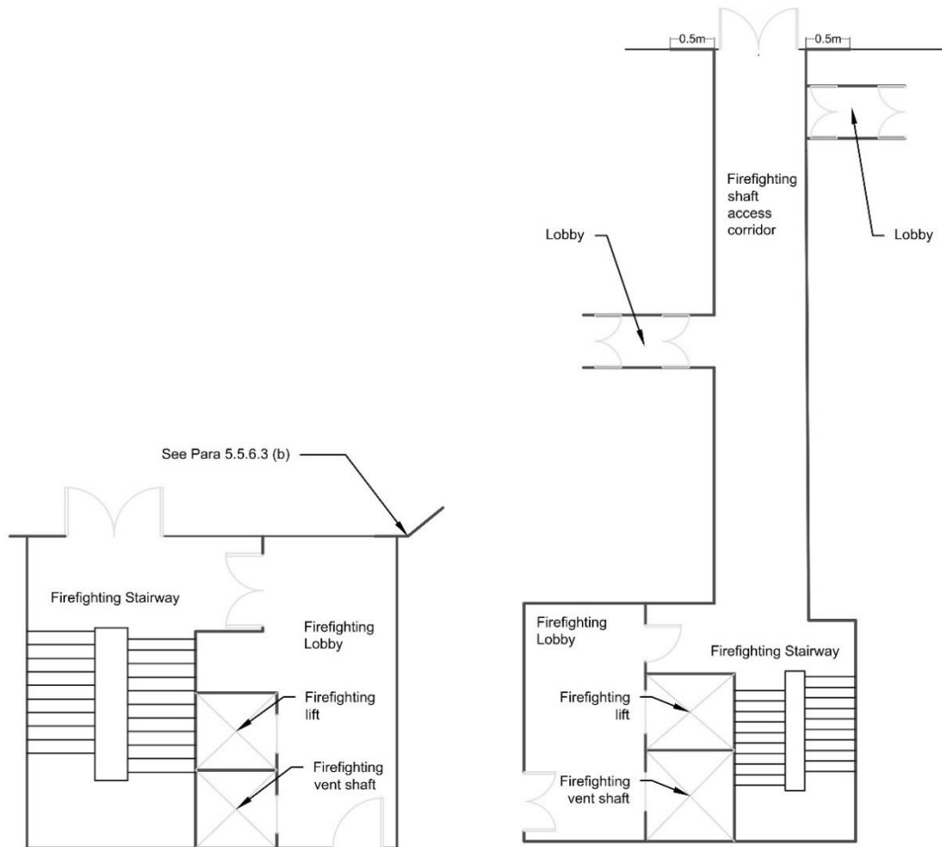
b. Firefighting shaft, access level, corridor access to firefighting shaft
