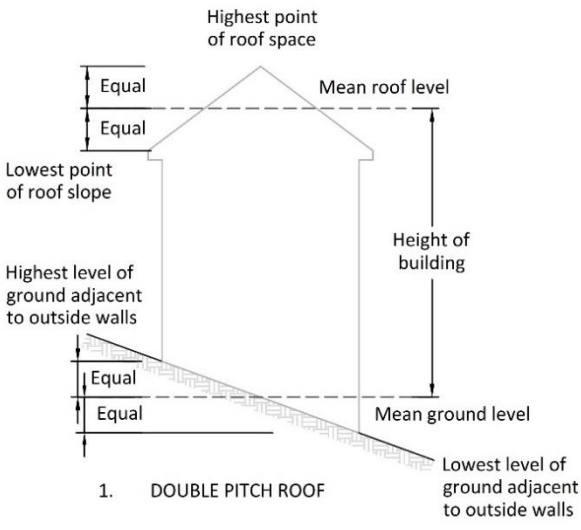
Diagram 90 Height of a Building
