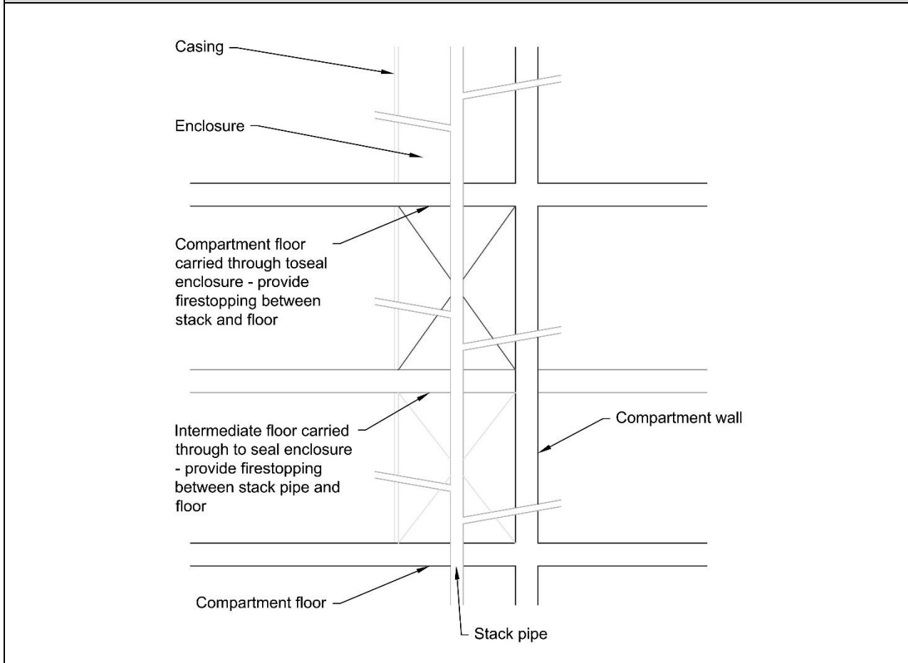
Diagram 84 Enclosures for Drainage or Water Supply Pipes
