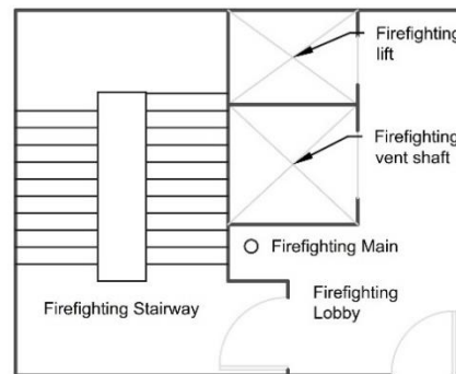
d. Firefighting shaft, accommodation level
