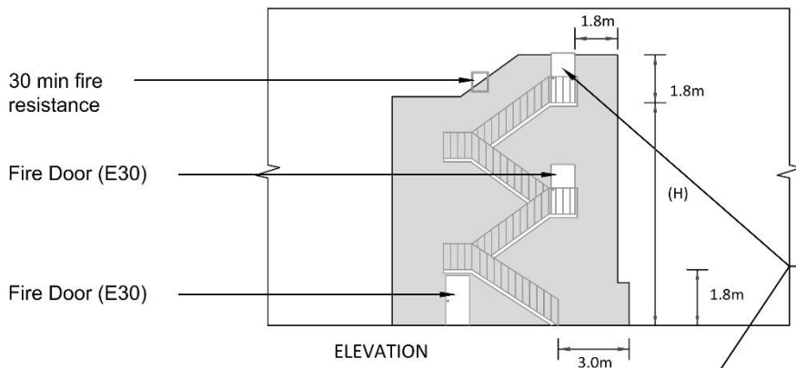
Diagram 17 External Escape Stairways
