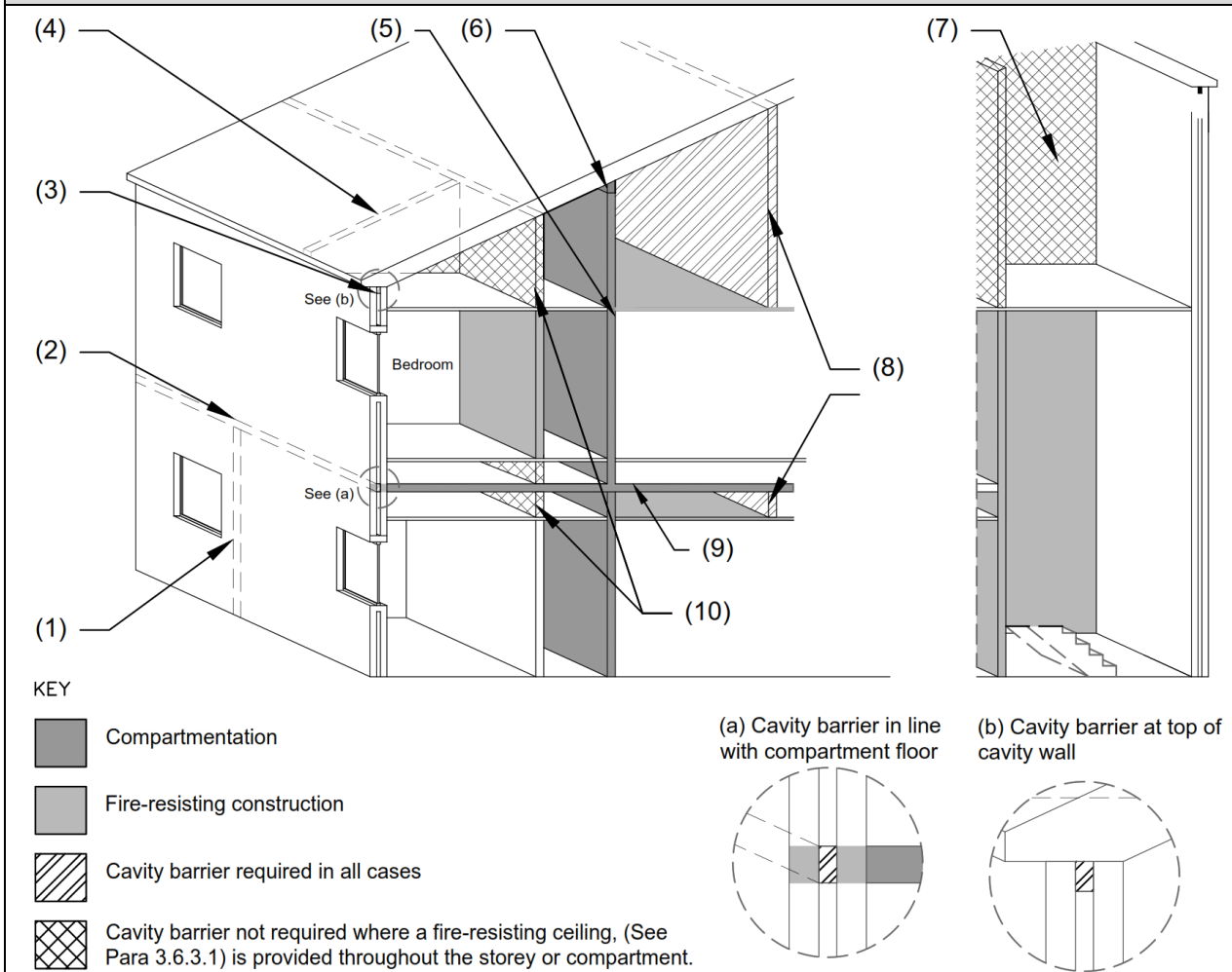
Diagram 53 Interrupting Concealed Spaces (Cavity Barriers)
