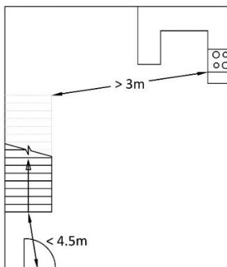
(b) Open plan arrangement for escape - stairway does not discharge into a kitchen
