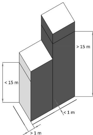
Example 1: Building containing flats (PG 1(c)) of differing heights, not divided by separating walls / not forming separated parts
