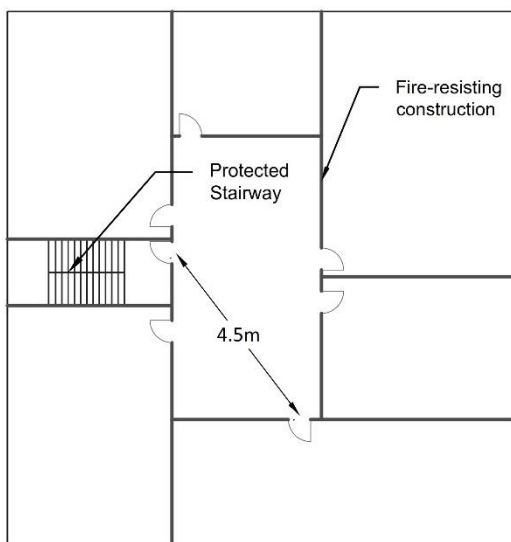
(a) Single stair building containing flats
