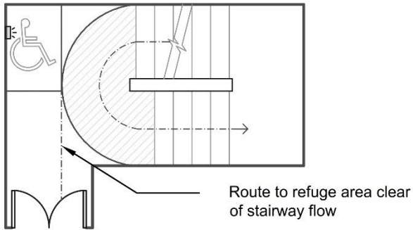
(a) Refuge in protected stairway, where access to the wheelchair space is counter (contra-flow) to the escape flow within the stairway
